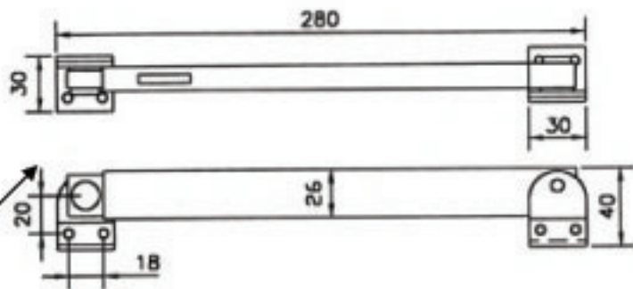
H-24-DL (left hand) & H-24-DR (right hand) H-24-DL (left hand) & H-24-DR (right hand)
