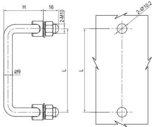
Folding Handles
