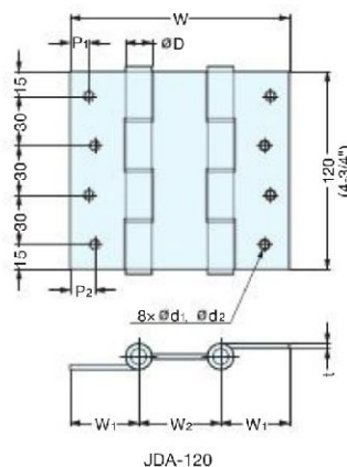
JDA-120
