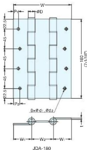
JDA-180
