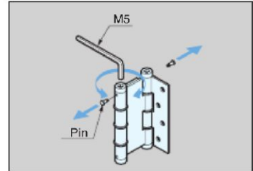
Spring Adjustment
