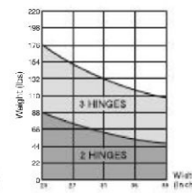
JDA-180-40A JDA-180-38S
