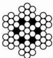
Cross section of 7x7 cable construction.
