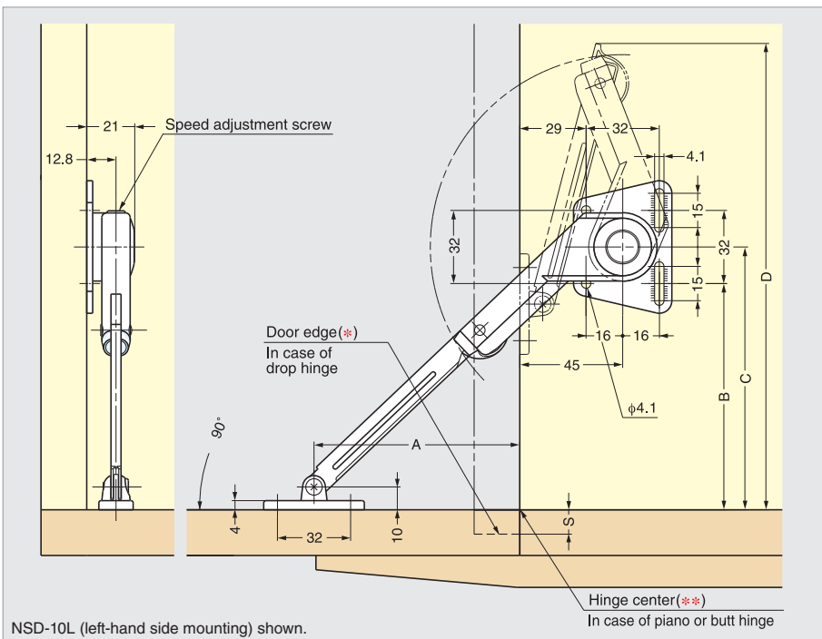
NSD-10L (left-hand side mounting) shown.
