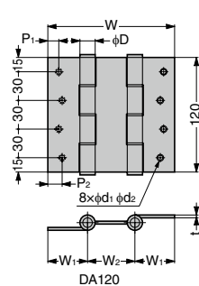
Hinges for double action door.
