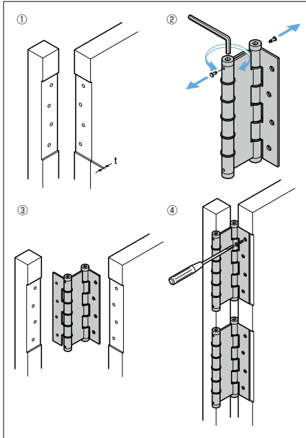
Hinges for double action door.
