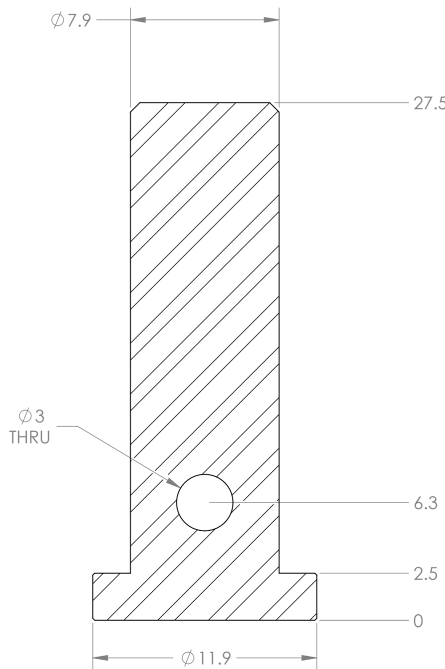
SECTION F-F
