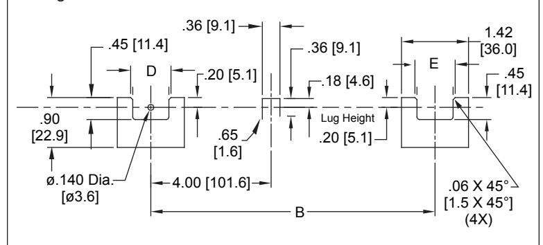
Drawer Cut-Out Recommendation
