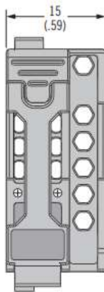
15 MM Housing
