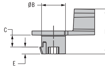
Slotted hole trigger / lever (R4-0-72894-X)
