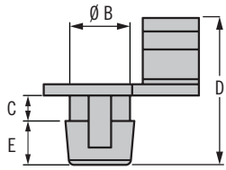
Round hole trigger / lever (R4-0-60784)
