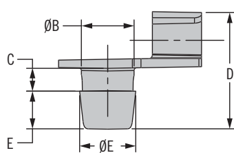
Round hole trigger / lever (R4-0-43922-X)
